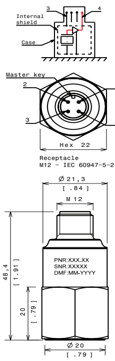
Fig 1c : Outline drawing B=3 (M12 Epoxy) electrical layout : See above B=2
