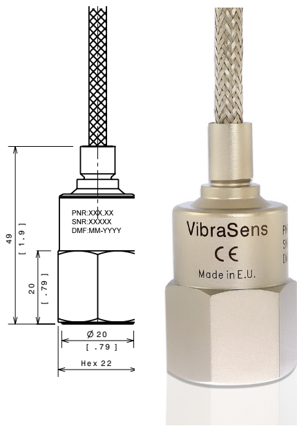
Fig 1e : Outline drawing B=7 (cable with overbraid) electrical layout : See above B=5
