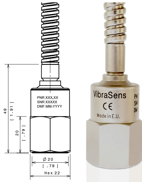
Fig 5 : Outline drawing B=8 (cable with conduit protection) electrical layout : See above B=5
